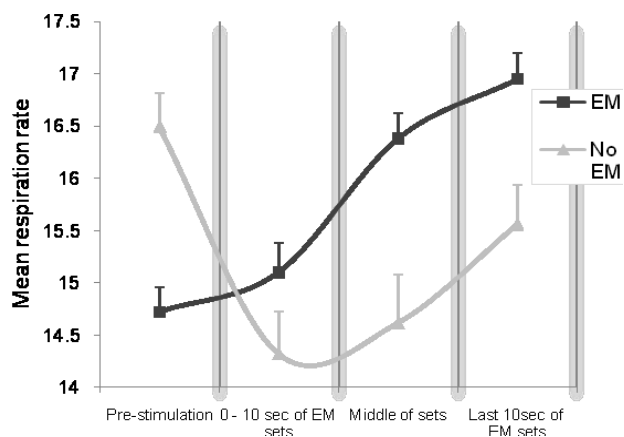
Figure 3. Mean respiration rate of each condition prior to and during eye movements of the first and last three sets of each session. Error bars represent SEM.
