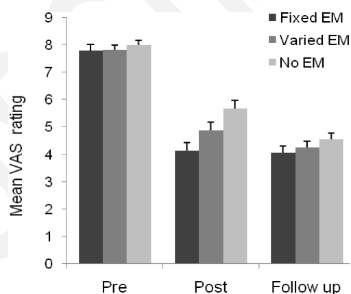
Figure 2. Mean VAS ratings for each condition at pre- and post-treatment and at follow up. Error bars represent SEM.
