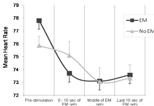
Figure 4. Mean heart rate of each condition prior to and during eye movements of the first and last three sets of each session. Error bars represent SEM.
