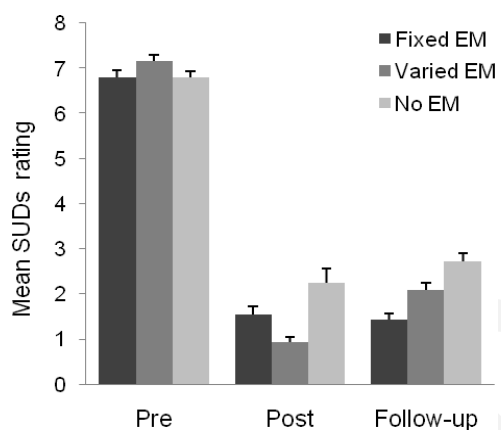
Figure 1. Mean SUDs ratings for each condition at pre- and post-treatment, and at follow-up. Error bars represent standard error of the mean (SEM).
